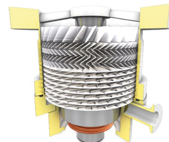
Turbomolecular pump
