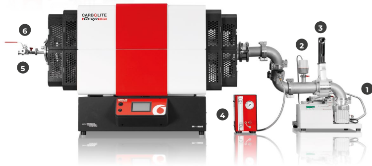
TS1 16/100/600 with turbo pump package and inert gas package
