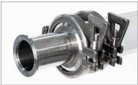
End seal with NW40 vacuum flange
