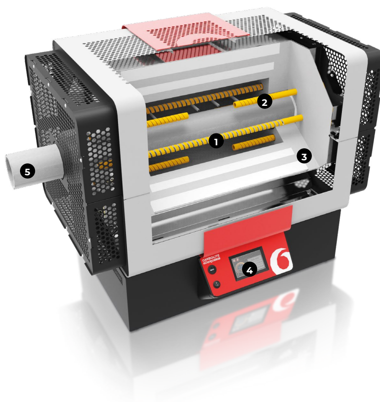
TF3 16/100/450 with CC-T1 controller
